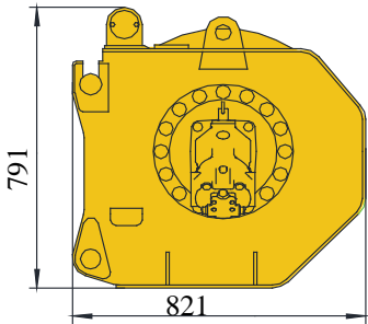
副起升机构 (含钢丝绳) 1409kg Auxiliary winch (rope included) 1409kg
